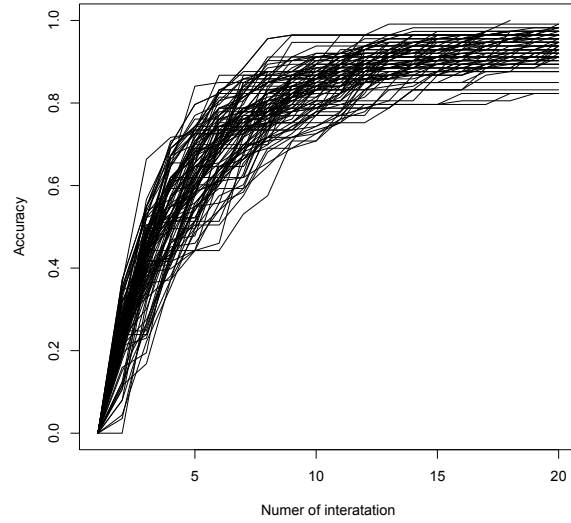
Figure 6: Cross-validated accuracy.
